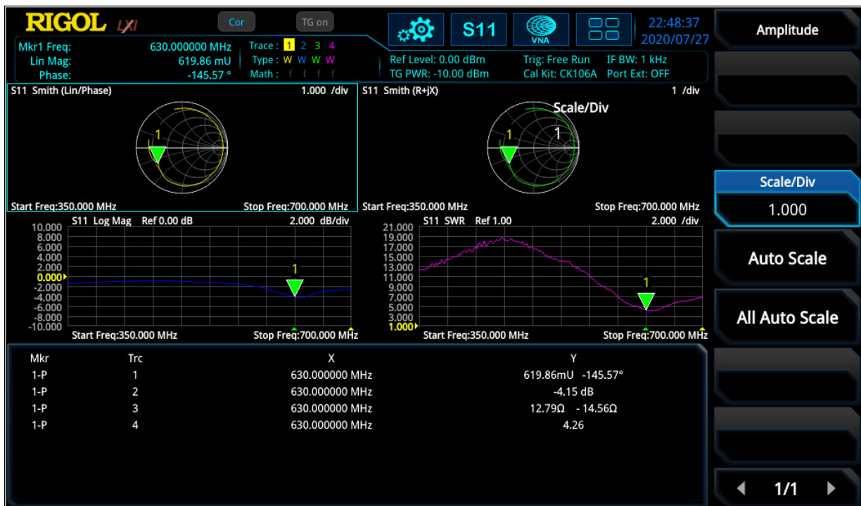
Figure 6: Different window of S_{11} parameter like smith- and Polar Plane, logarithm. Magnitude and SWR
